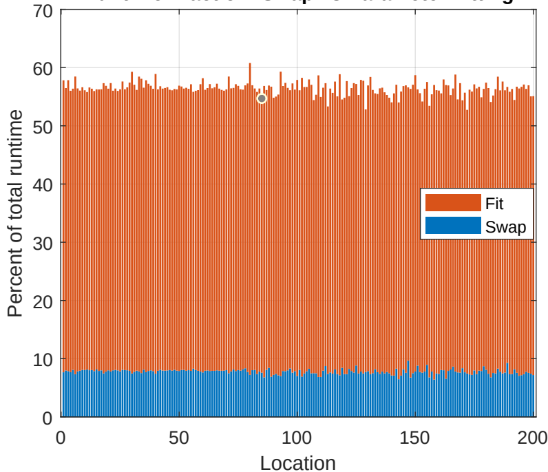
Runtime Fraction: Swap vs Parameter Fitting
